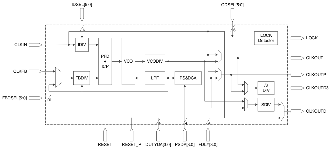
图 3-42 PLL 示意图(GW1N-1/GW1N-1S/GW1N-4/GW1N-9)
