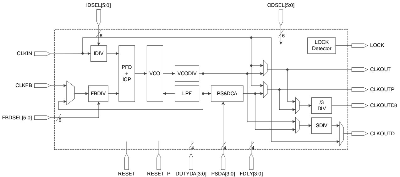
图 3-16 PLL 示意图(GW1N-4)
