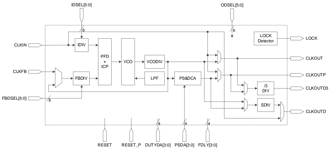
Figure 3-37 PLL Structure
