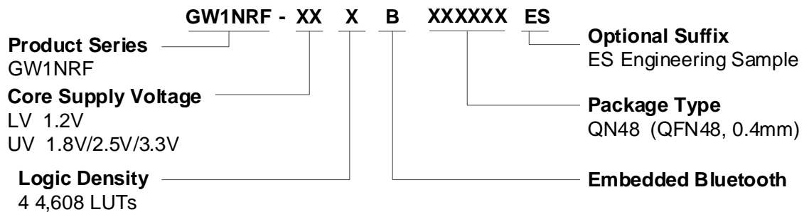
Figure 5-1 Part Naming-ES
