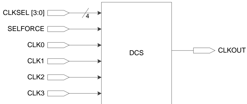
Figure 3-34 DCS Concept
