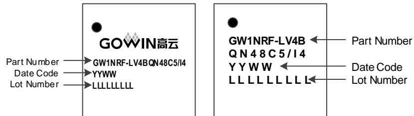
Figure 5-3 Package Mark
