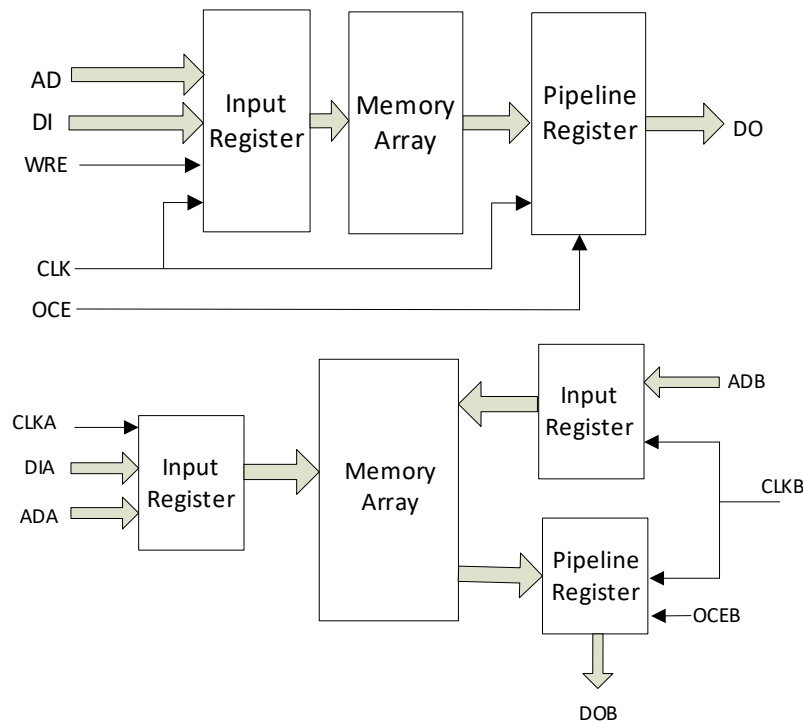
Figure 2-11 Pipeline Mode in Single Port, Dual Port, and Semi-Dual Port Mode
