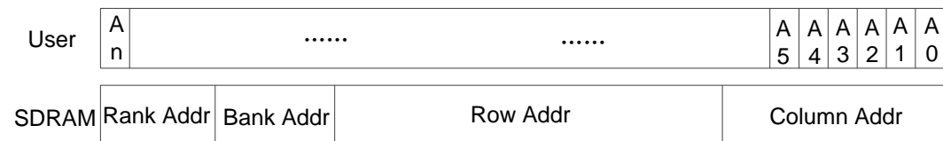
图 4-4 Rank-Bank-Row-Column 顺序的寻址方案
