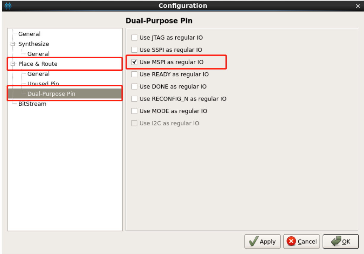
图 3-31 Dual-Purpose Pin 配置
