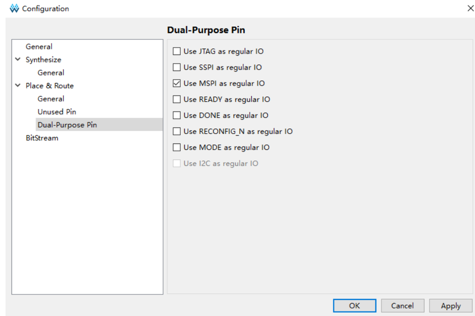
图 4-3 配置 Dual-Purpose Pin 选项
