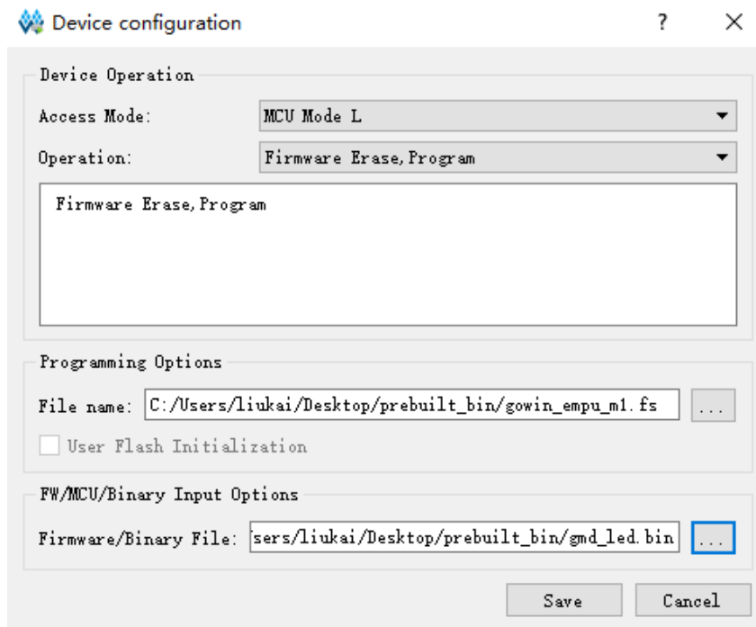
图 5-3 GW1N(R)-9C Device Configuration
