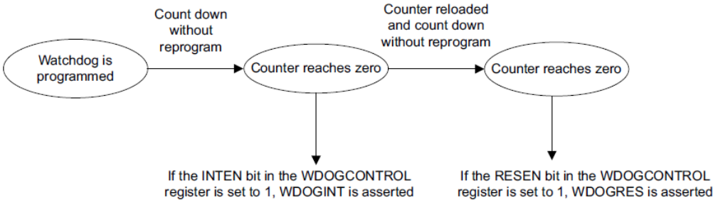
图 6-1 Watch Dog Operation
