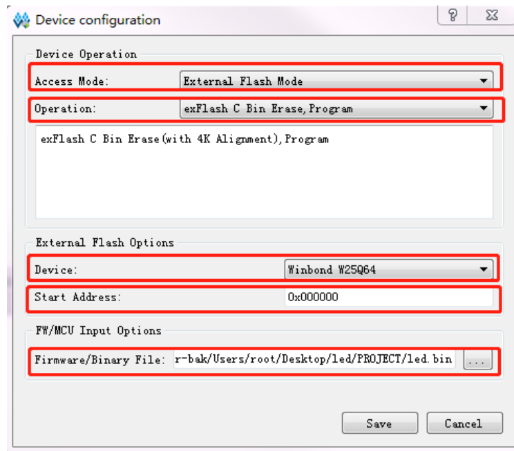
图 2-4 Device configuration
