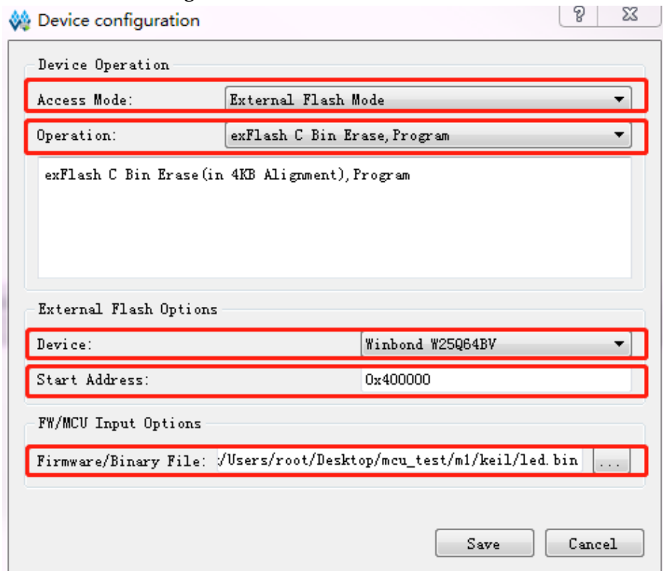
图 2-4 Device configuration
