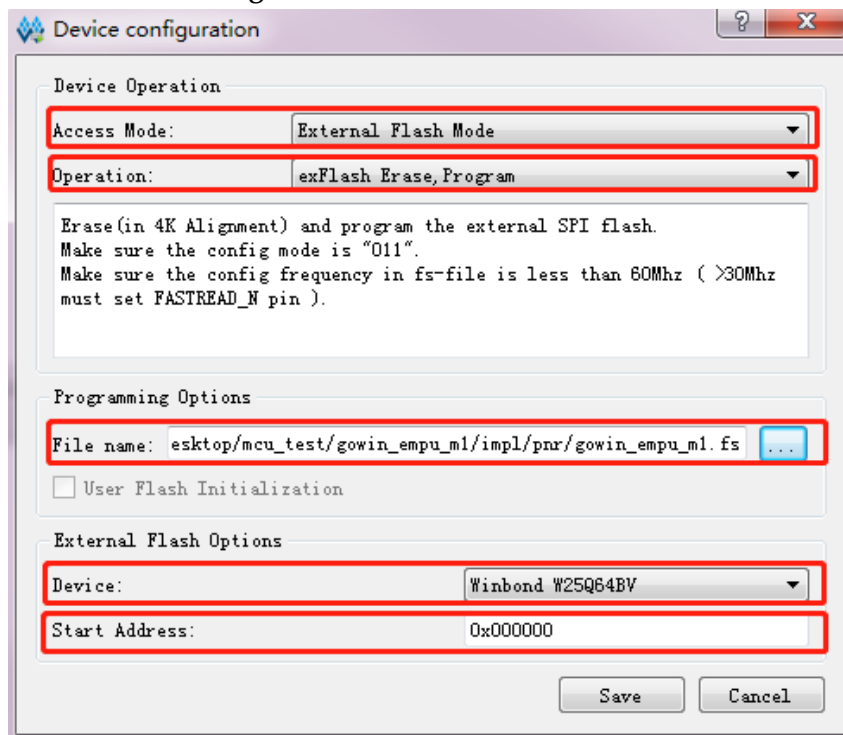
图 3-4 Device configuration
