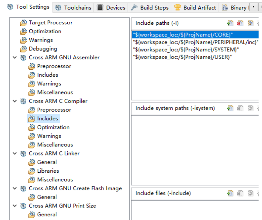
图 2-6 配置 Cross ARM C Compiler > Includes
