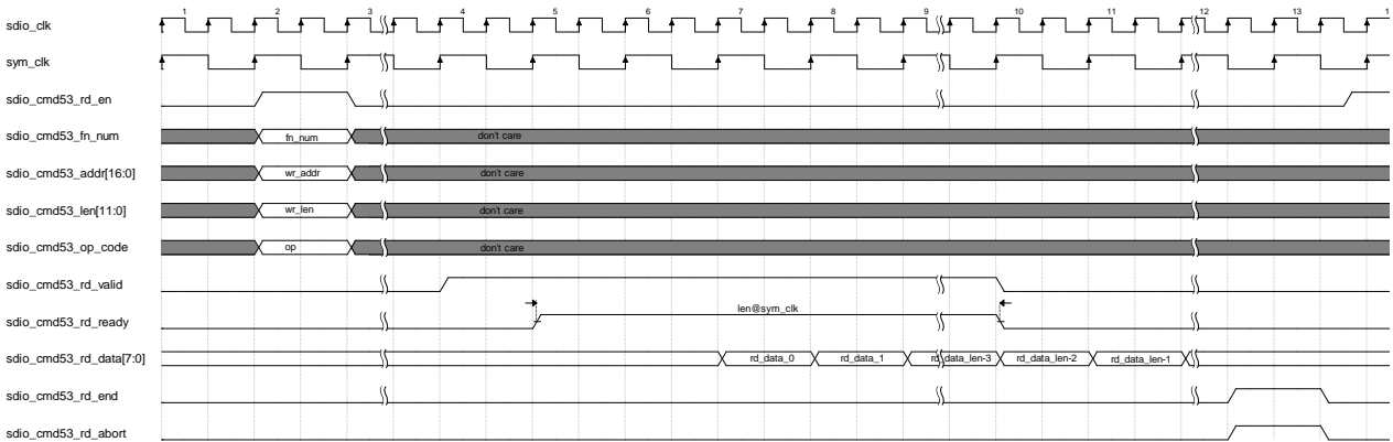
图 4-18 Read Good Abort Case1
