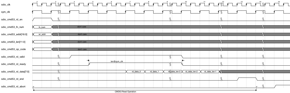
图 4-19 Read Good Abort Case2
