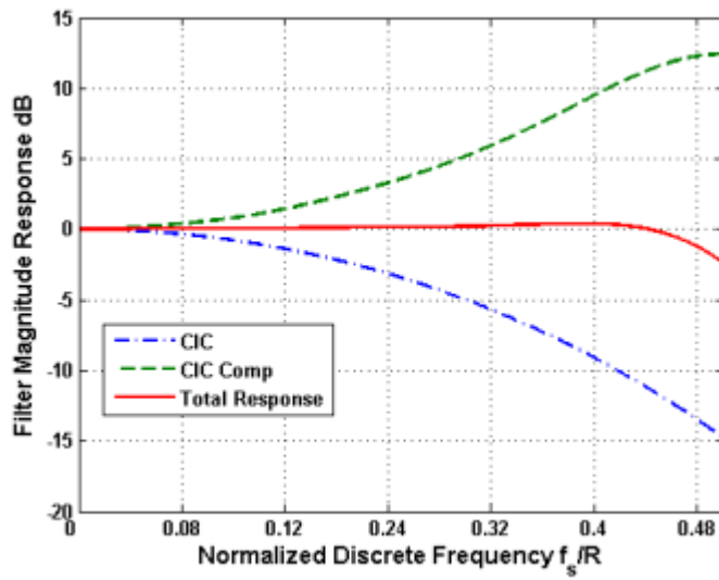
图 2-4 CIC Compensation Filter
