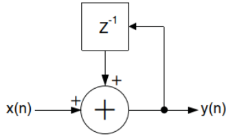
图 2-2 Integrator Filter
