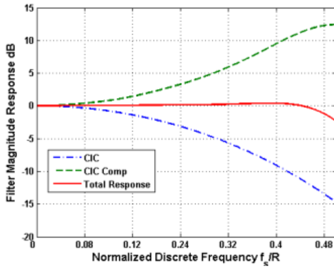
图 2-4 CIC Compensation Filter
