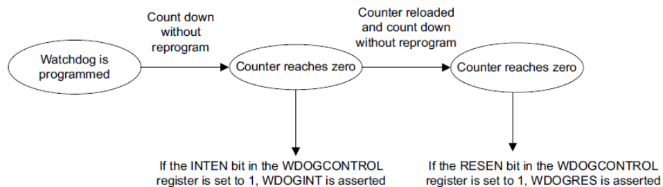
图 6-1 WatchDog Operation
