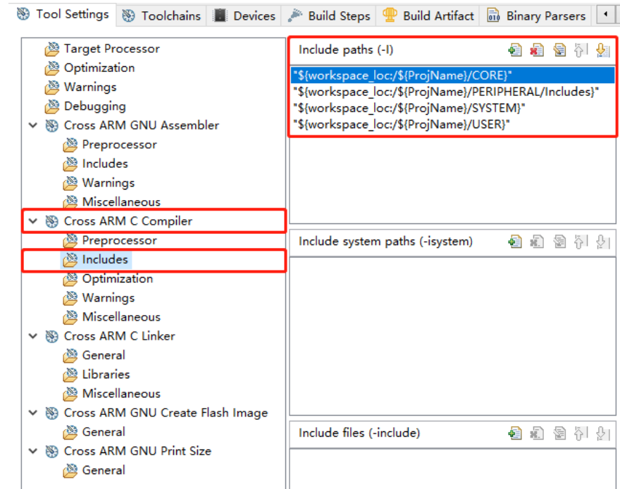
图 2-6 配置 Cross ARM C Compiler > Includes 选项
