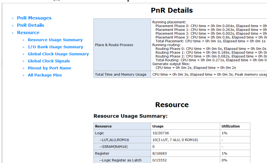
图 6-2 Place & Route Report
