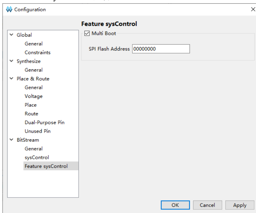
图 4-34 非 GW5A(S)(T)-138/GW5A(S) (R)-25/GW5AT-60/GW5AT-75 器件 Feature sysControl 选项
