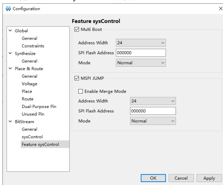
图 4-35 GW5A(S)(T)-138/GW5A(S) (R)-25/GW5AT-60/GW5AT-75 器件 配置 Feature sysControl 选项
