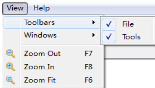
图 3-30 View 菜单
