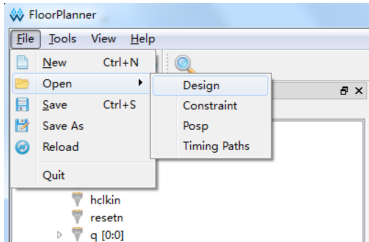
图 3-10 File 菜单
