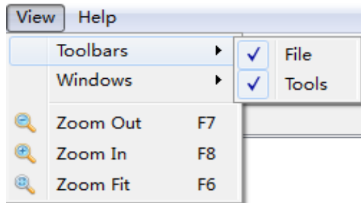
图 3-30 View 菜单
