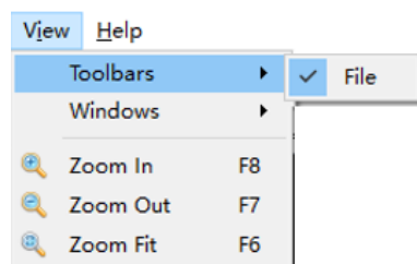
图 3-23 View 菜单
