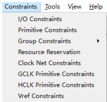
图 3-7 Constraints 菜单
