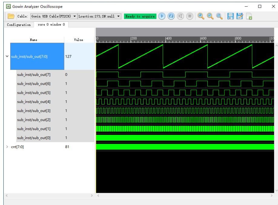
图 4-13 Unsigned Line Chart
