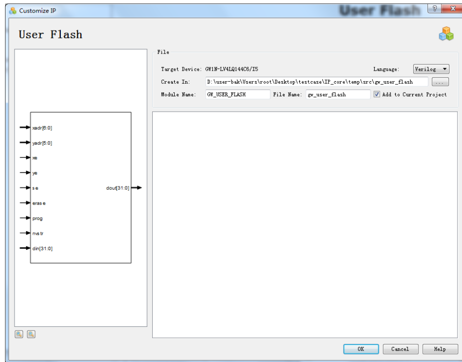
图 3-104 User Flash IP Customization 设置
