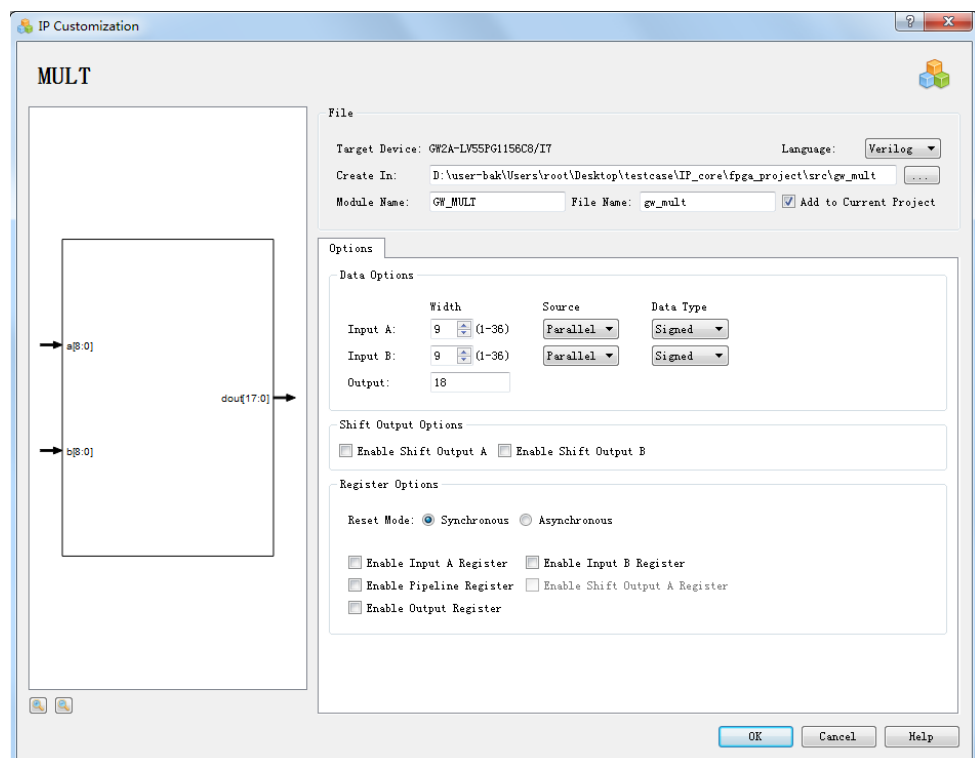
图 3-49 MULT IP Customization 设置
