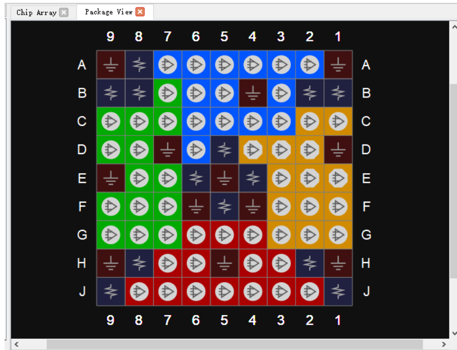
图 3-44 GW1N-9-WLCSP81M Top View
