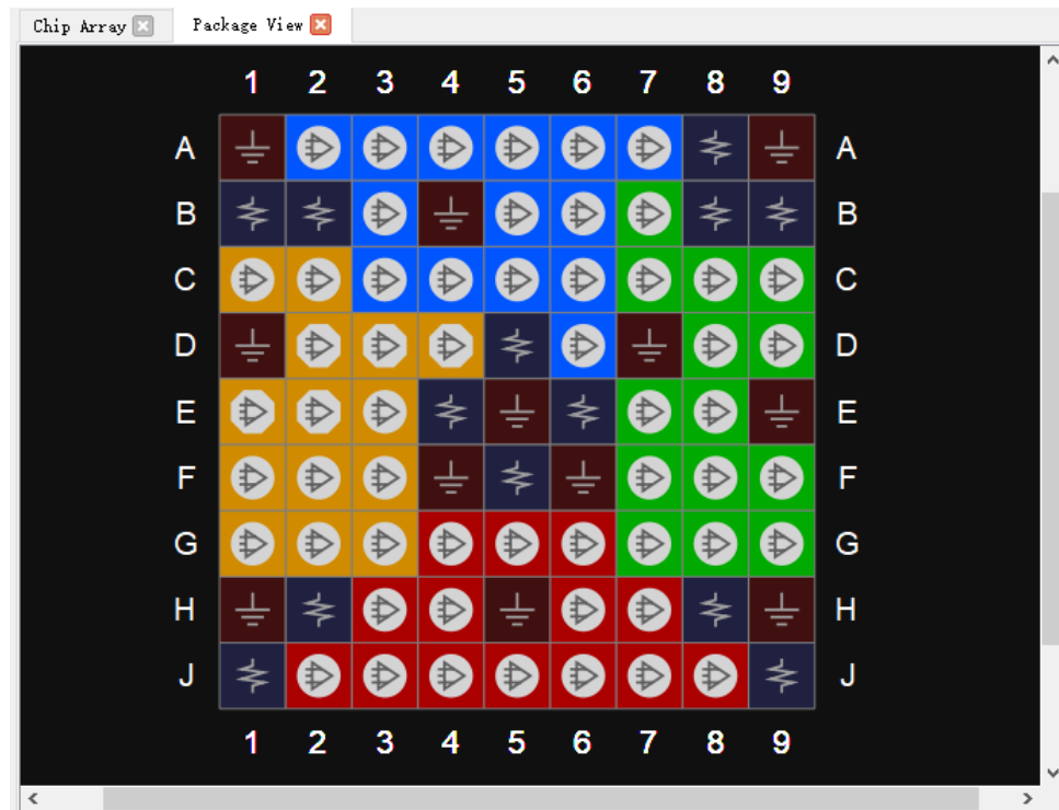
图 3-38 GW1N-9-WLCSP81M Bottom View
