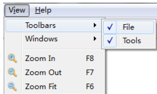
图 3-24 View 菜单
