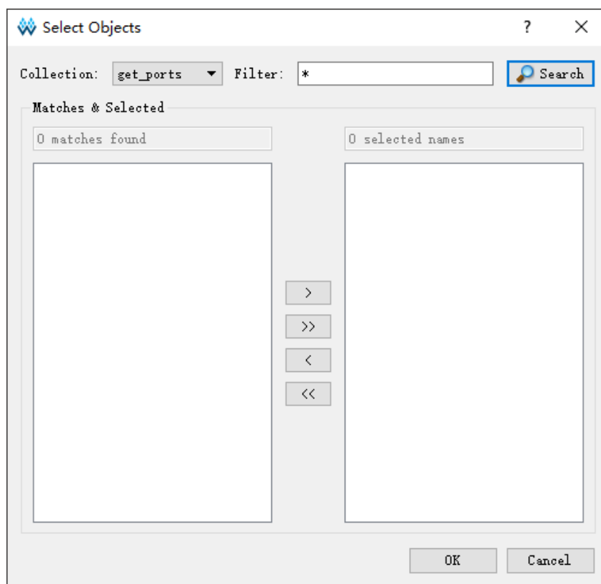
Figure 4-14 Select Objects
