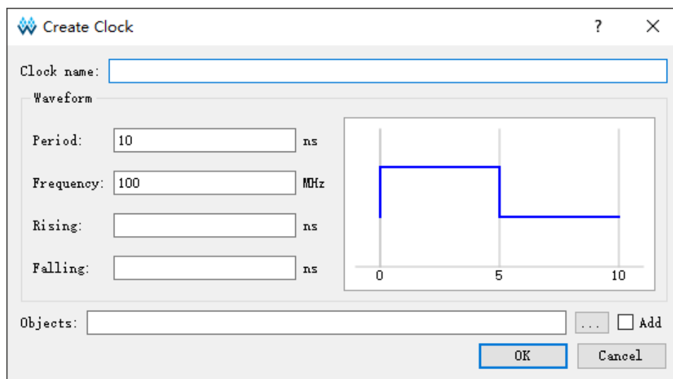
Figure 4-13 Create Clock
