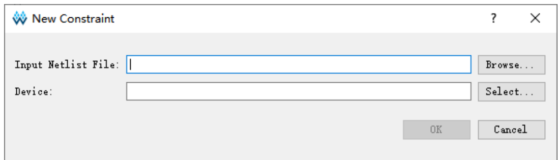
Figure 4-8 New Constraint
