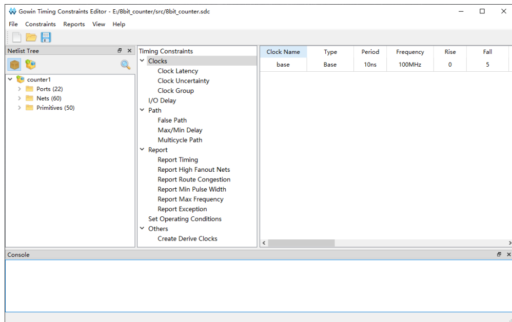
Figure 4-5 Timing Constraint Editor Interface
