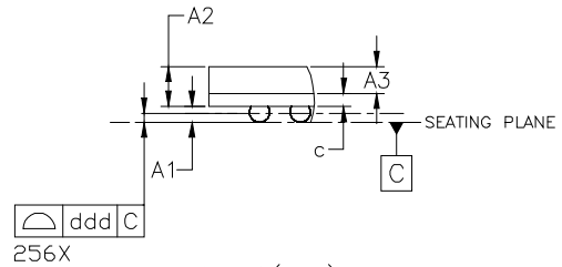
DETAIL A(2:1)
