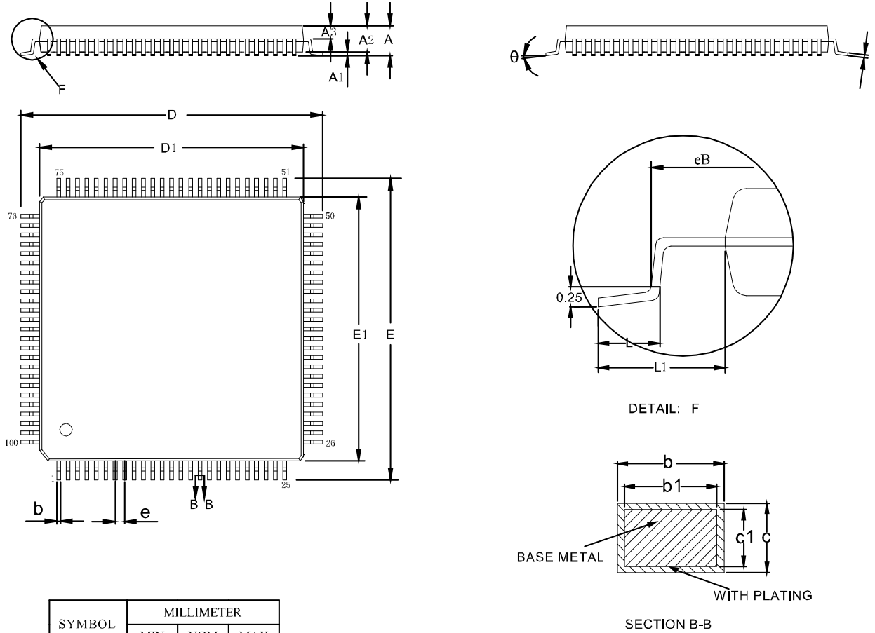
图 4-9 封装尺寸 LQ100/LQ100X-LV/LQ100X-UV
