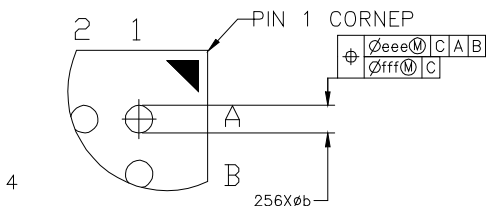
DETAIL B(3:1)
