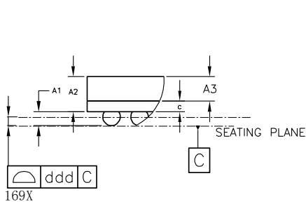
DETAIL A(2:1)
