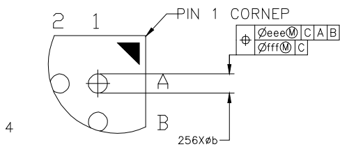
DETAIL B(3:1)
