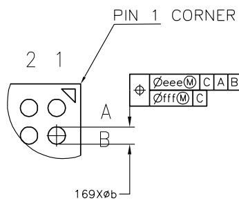
DETAIL B(2:1)
