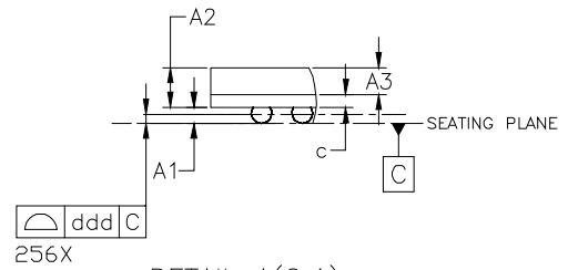
DETAIL A(2:1)
