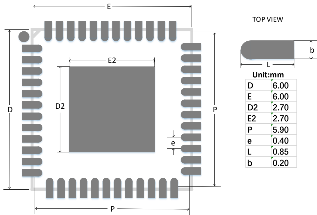
图 4-24 推荐 PCB Layout QN48/QN48F(GW1N-9)
