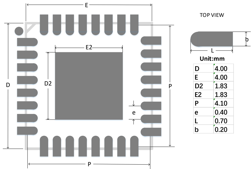
图 4-14 推荐 PCB Layout FN32(GW1N-1S)
