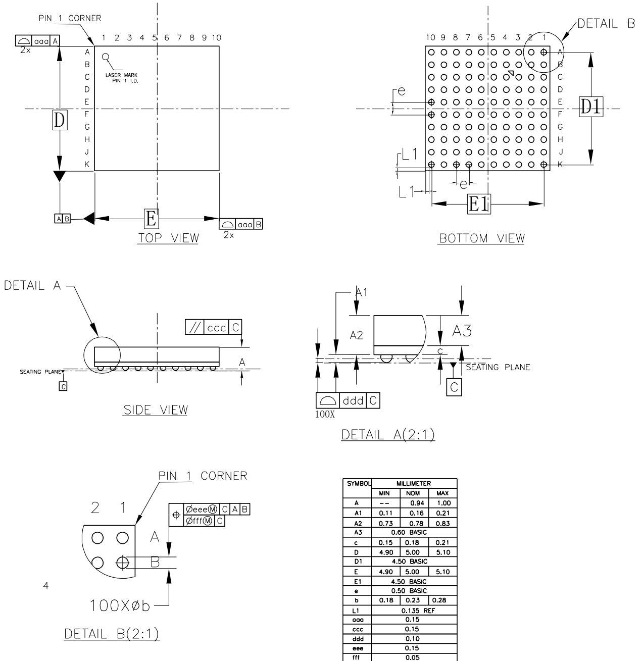
图 4-4 封装尺寸 MG100P/MG100PF/MG100PA/ MG100PT/MG100PS
