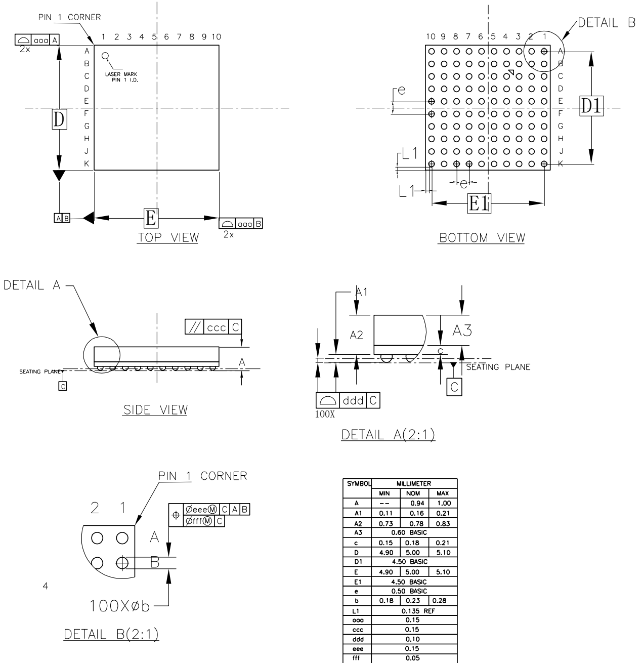
图 4-5 封装尺寸 MG100P/MG100PF/MG100PA/ MG100PT/MG100PS
