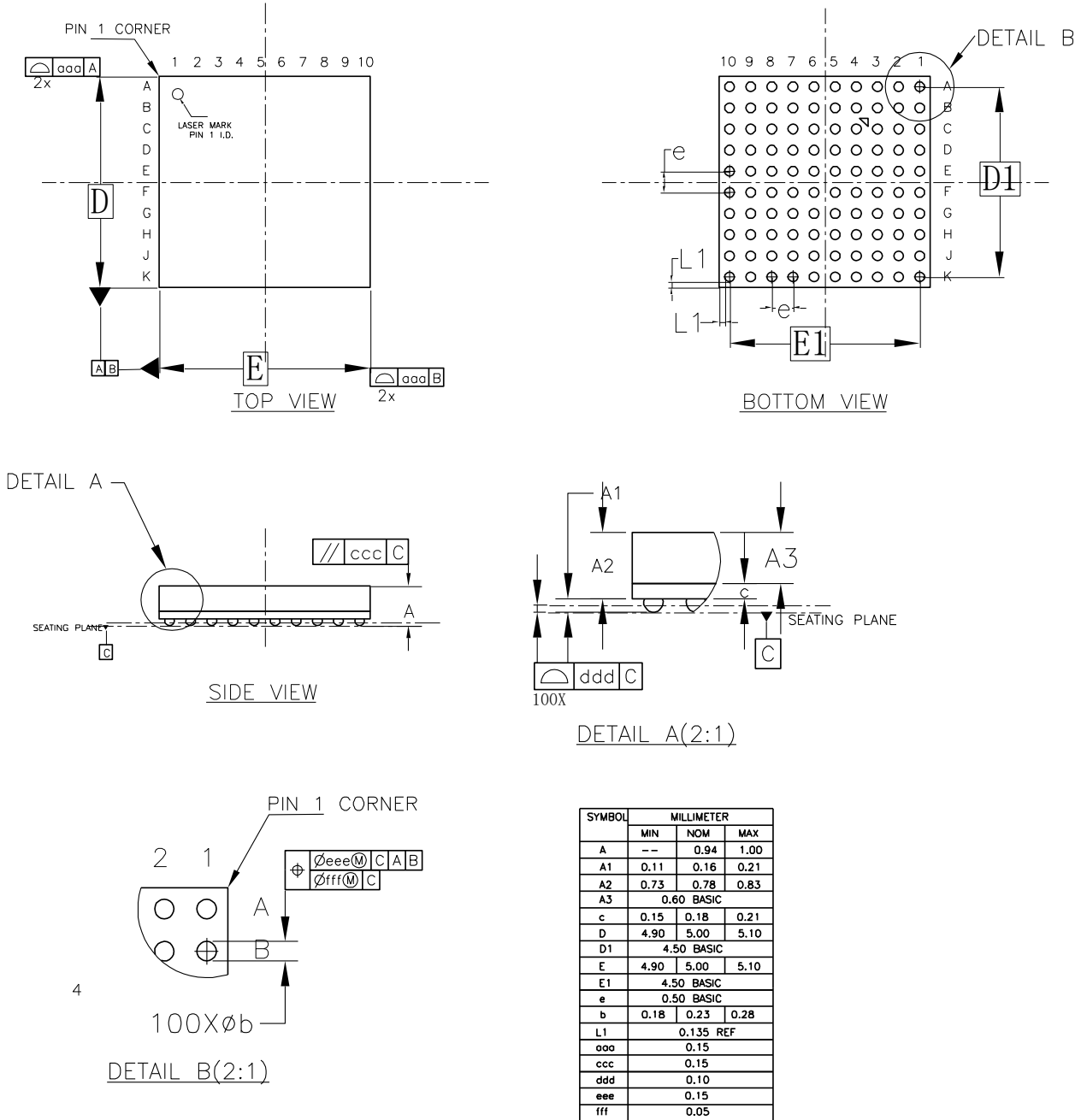
图 4-7 封装尺寸 MG100P/MG100PF/MG100PA/ MG100PT/MG100PS
