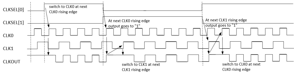
图 3-5 DCS mode: RISING 时序图
