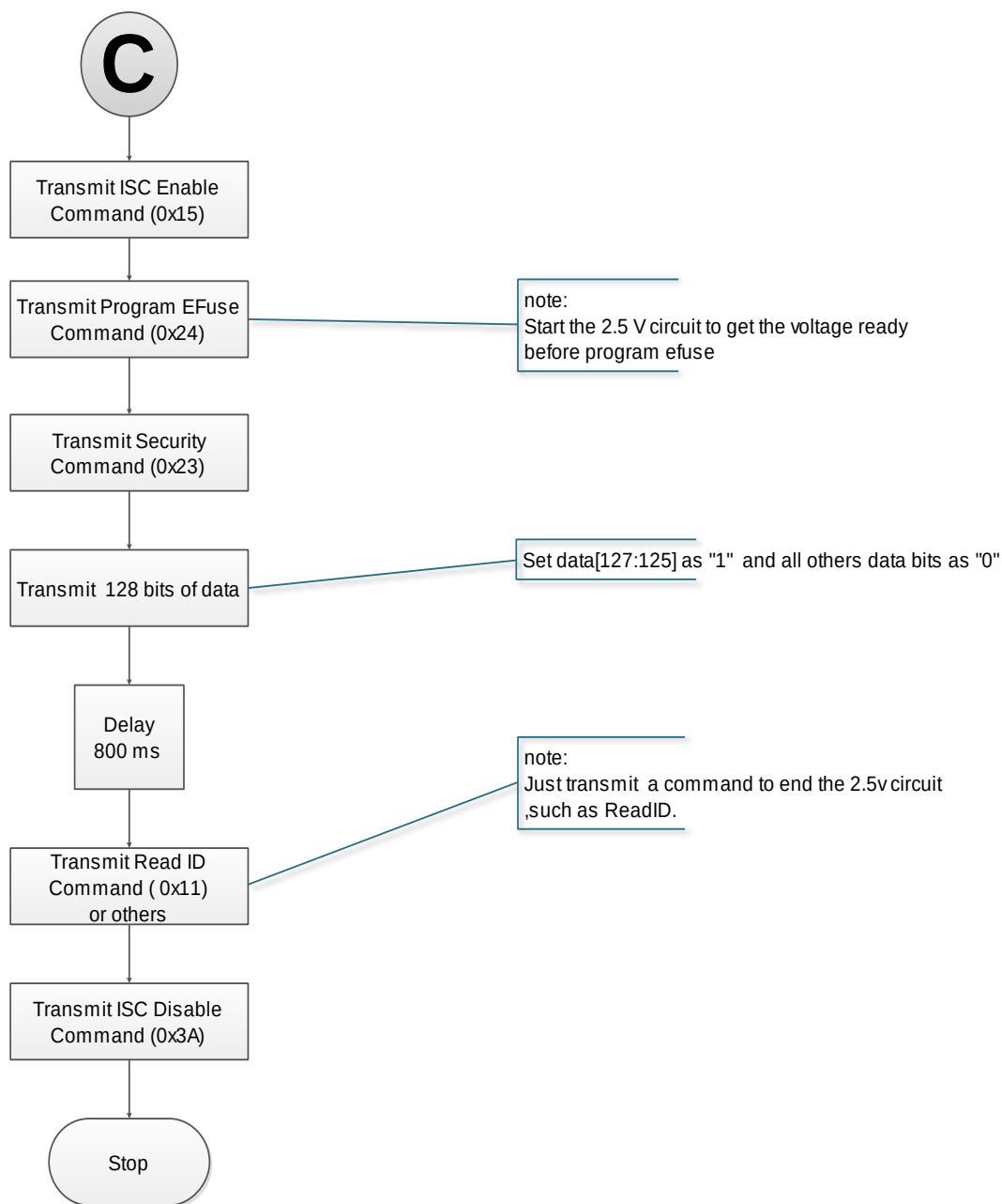
图 7-8 Lock AES Key Flow
