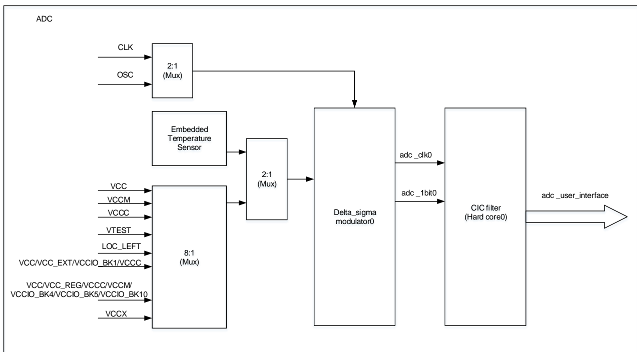
Figure 2-1 ADC Structure Diagram For 25K devices
