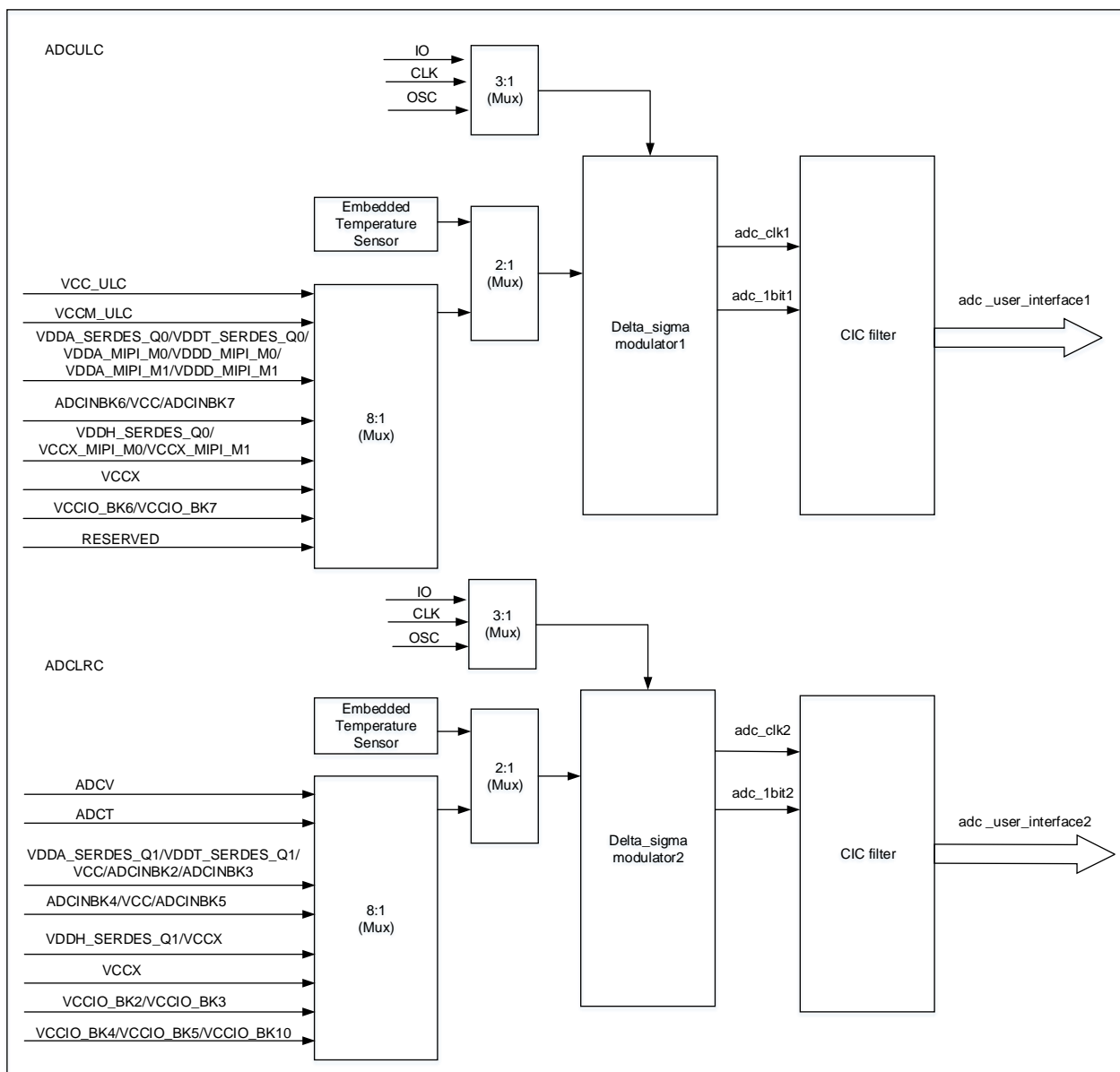
Figure 2-2 ADC Structure Diagram For 138/75K devices
