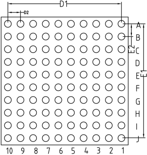
BOTTOM VIEW Ball Up
