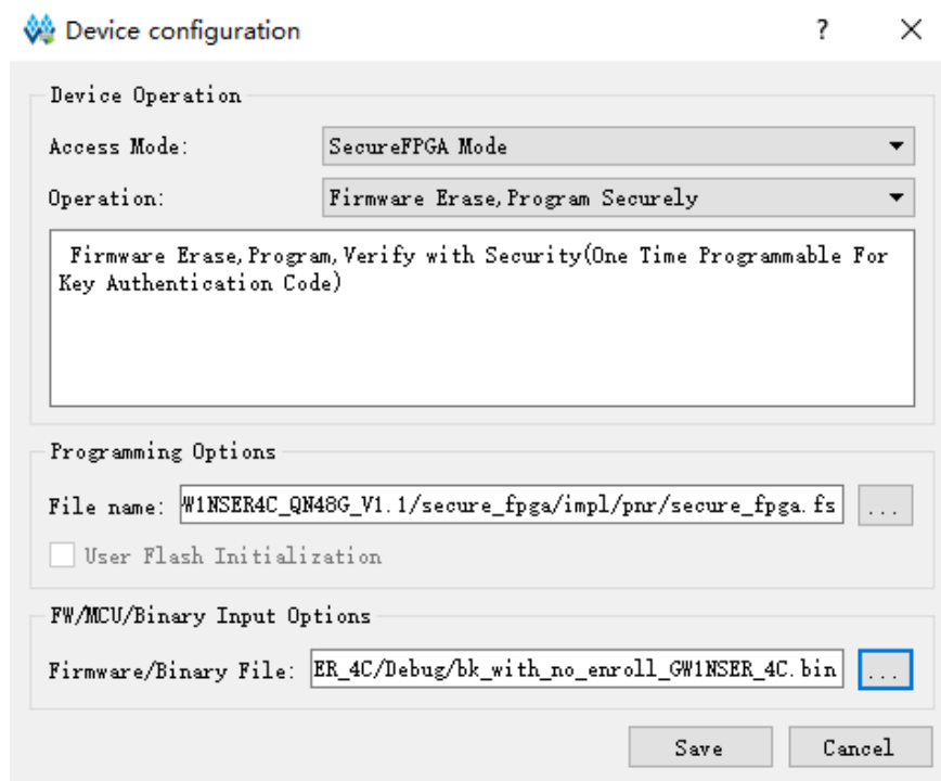
图 2-7 GW1NSER-4C (Gowin_EMPU(GW1NS-4C))下载属性配置
