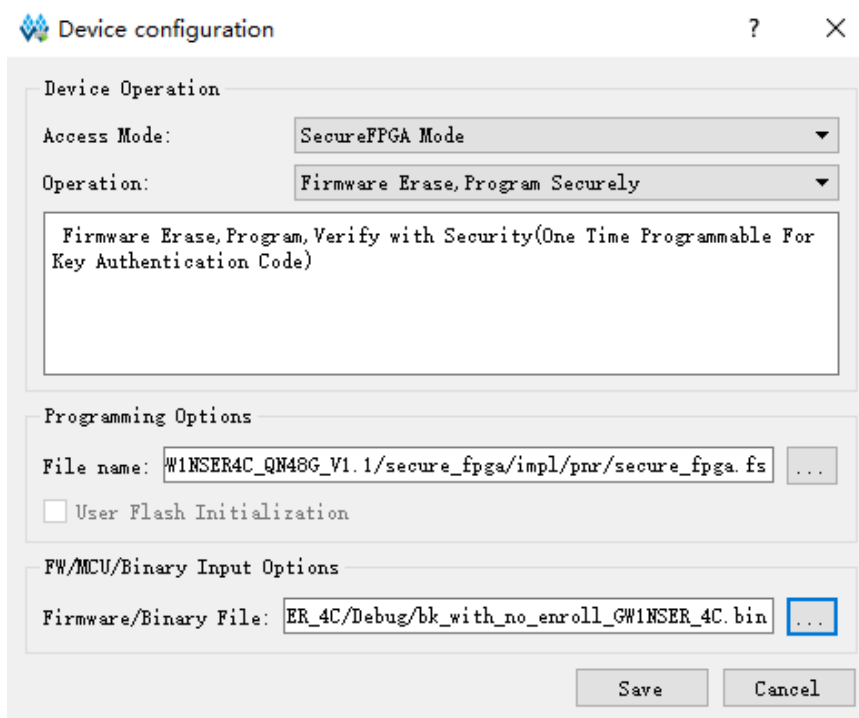
图 3-10 GW1NSER-4C (Gowin_EMPU(GW1NS-4C))下载属性配置
