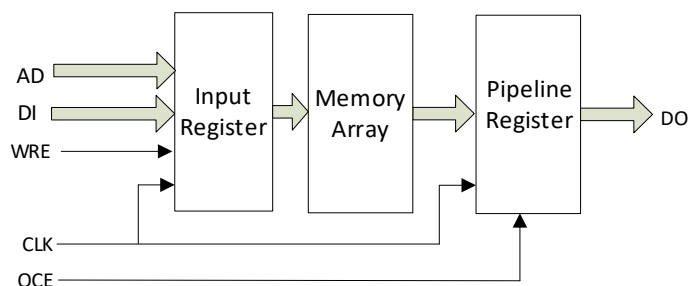
Figure 2-11 Pipeline Mode in Single Port Mode, Dual Port Mode, and Semi-dual Port Mode
