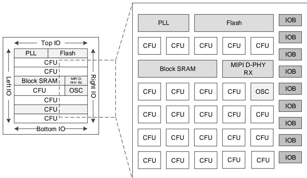
Figure 2-2 Architecture Overview of GW1NZ-2
