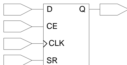
Figure 2-10 I/O Register Diagram
