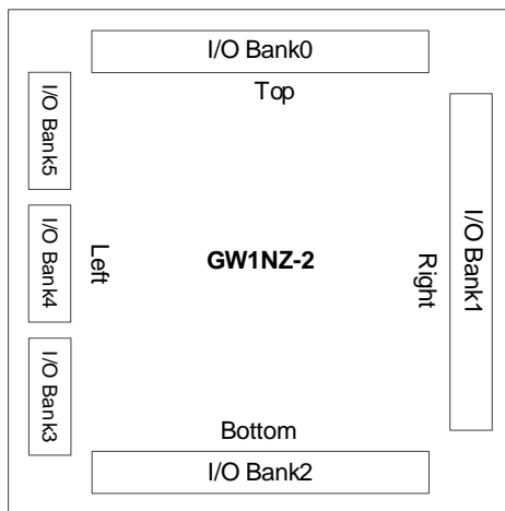
Figure 2-6 I/O Bank Distribution View of GW1NZ-2
