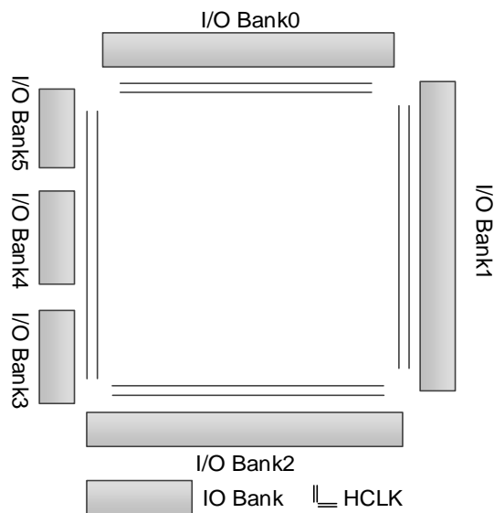
Figure 2-16 GW1NZ-2 HCLK Distribution
