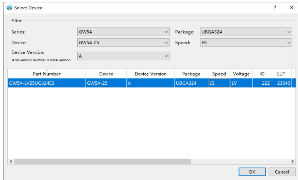
图 3-3 Select Device
