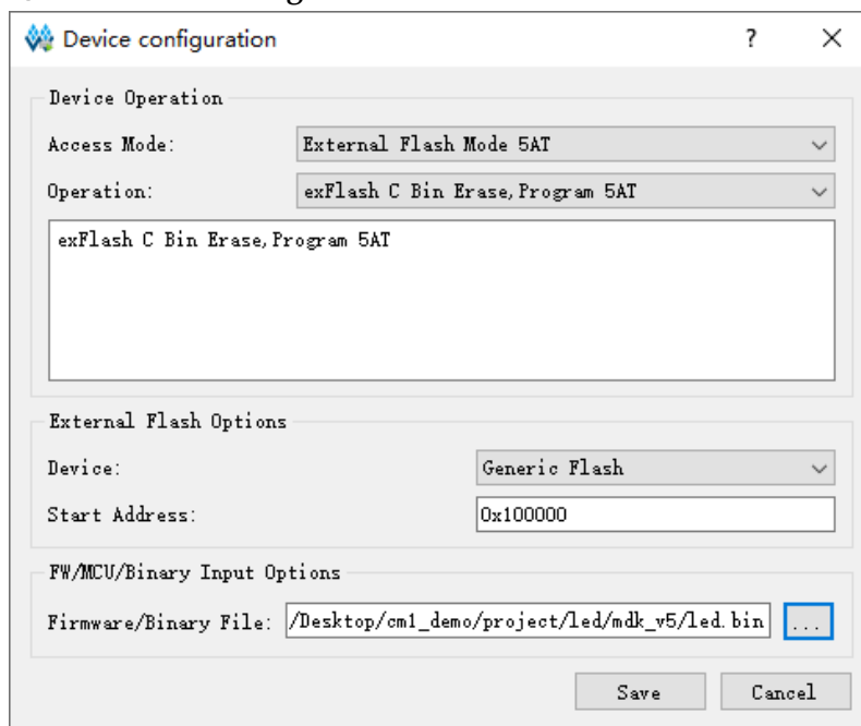
图 2-4 Device configuration
