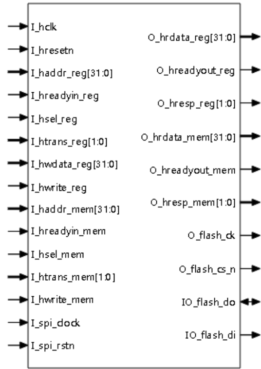
图 3-2 Gowin SPI Nor Flash Interface (With Internal Flash) IP IO 端口示意图
