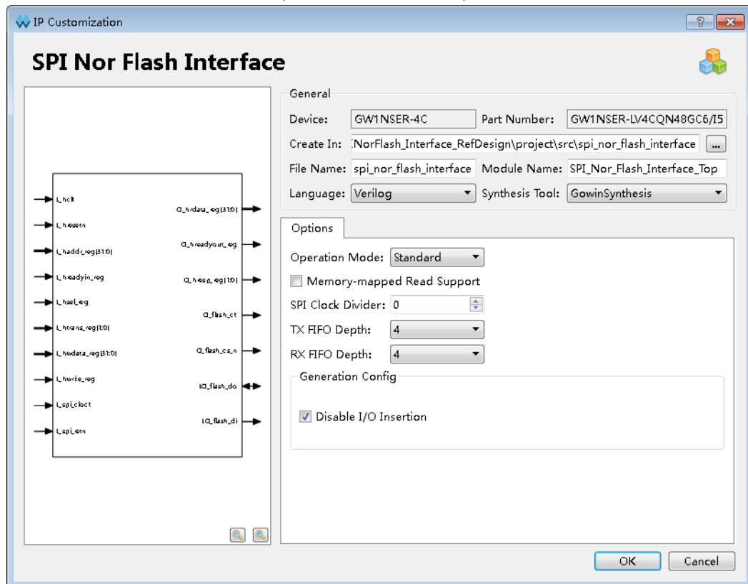
图 4-3 SPI Nor Flash Interface (With Internal Flash) IP 核接口示意图
