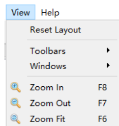
图 3-24 View 菜单
