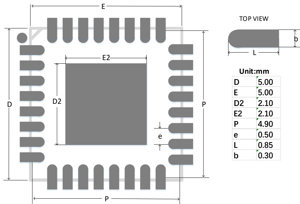
图 4-16 推荐 PCB Layout QN32(GW1N-1/4)
