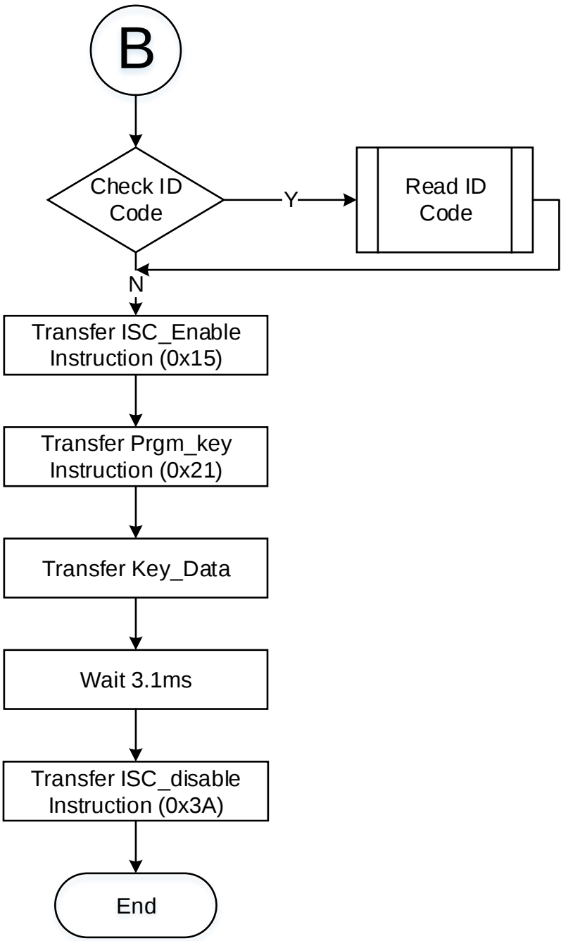
图 4-12 Program AES Key Flow
