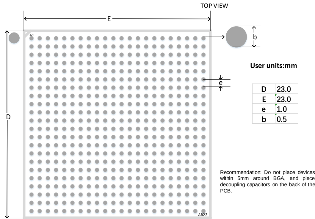
图 4-14 推荐 PCB Layout PG484A (GW5AT-138)
