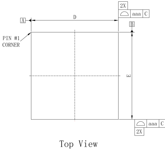
图 4-21 封装尺寸 UG225H (GW5AT-60)
