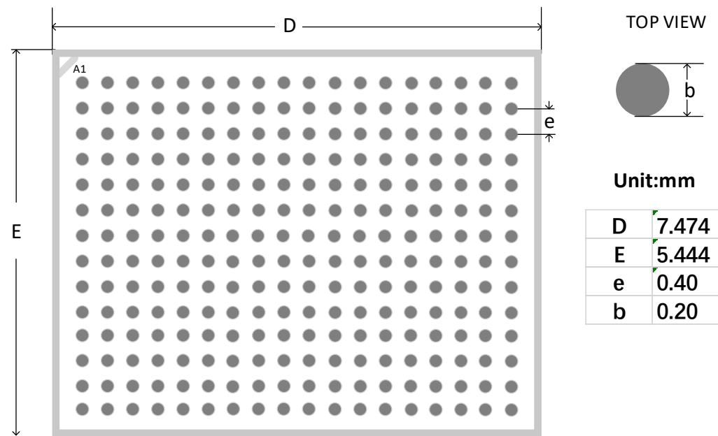
图 4-4 推荐 PCB Layout CS234 (GW5AT-60)
