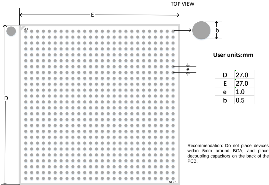
图 4-6 推荐 PCB Layout FPG676A (Flip Chip, GW5AT-138)
