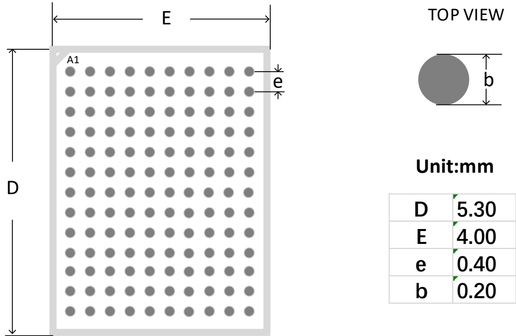
图 4-2 推荐 PCB Layout CS130/CS130F (GW5AT-15)
