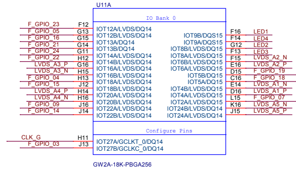
GW2A-18K-PBGA256
