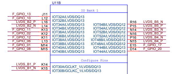
GW2A-18K-PBGA256
